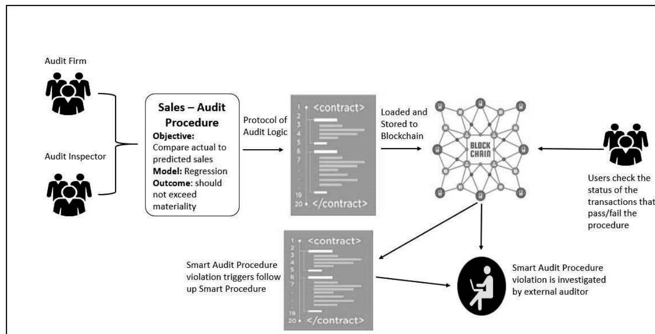
FIGURE 1 Smart Audit Procedure for Sales (Adapted from Rozario and Vasarhelyi 2018)
